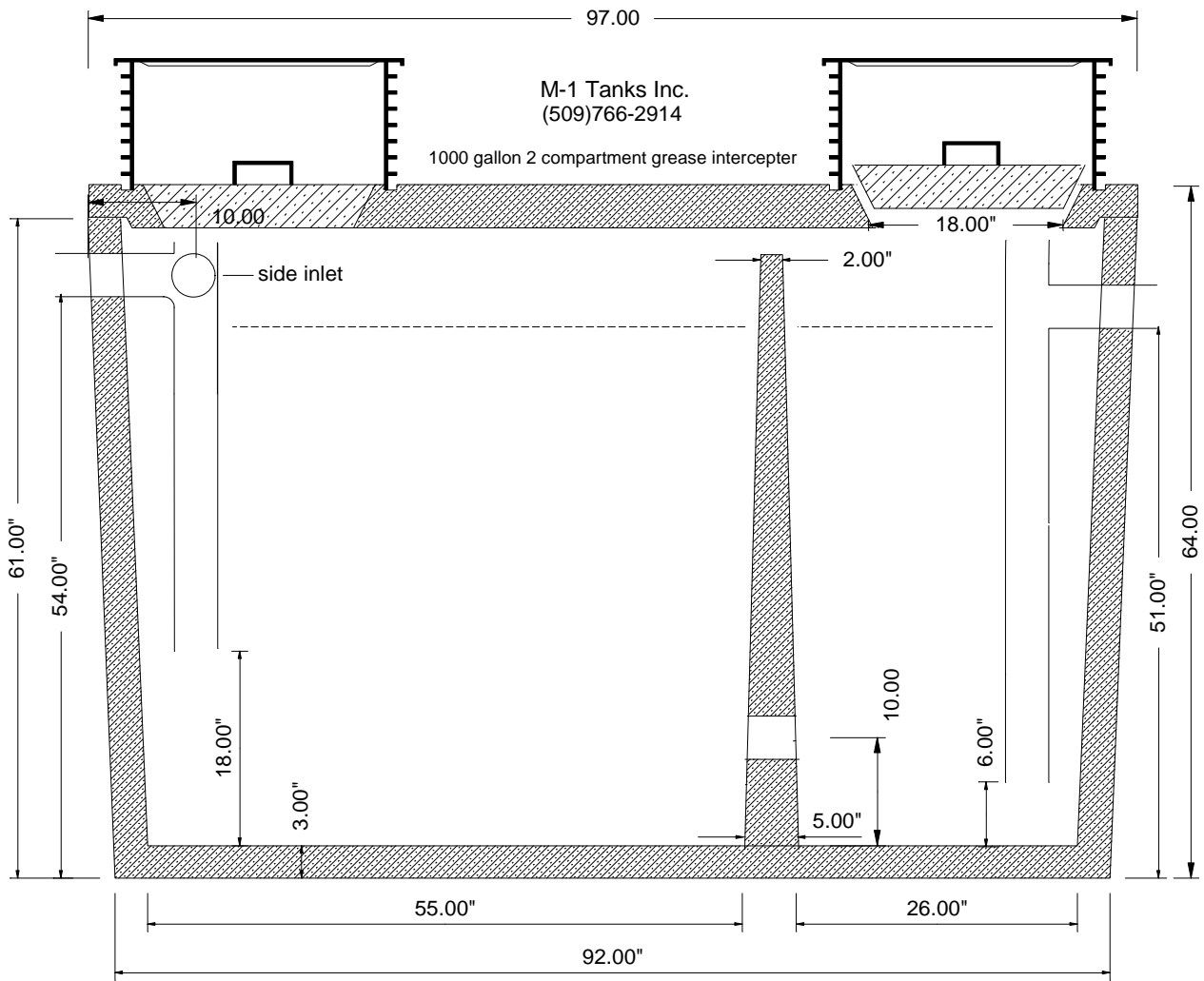
Cross Section
