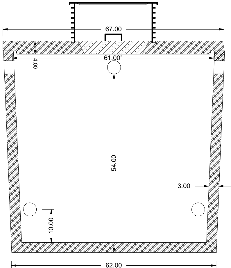
Cross Section
